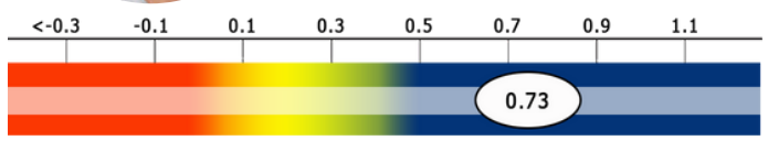
Effect Size
