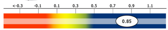
Effect Size
